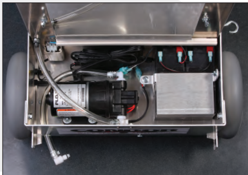
The Condor has an easy access compartment that houses the pump and battery charger, stowed on-board.
